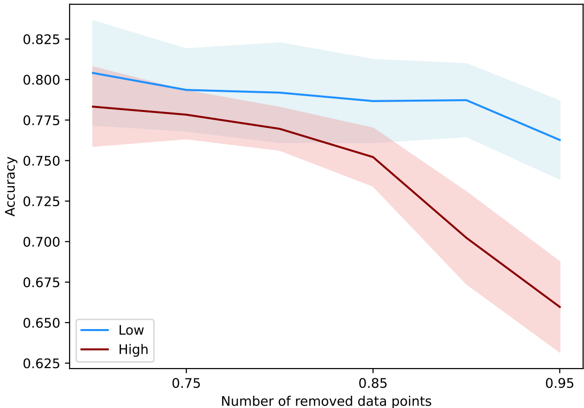
DataAttrOpt(5000, 0.02, 15, max+s, alpha=0.5) - imdb-embeddings
